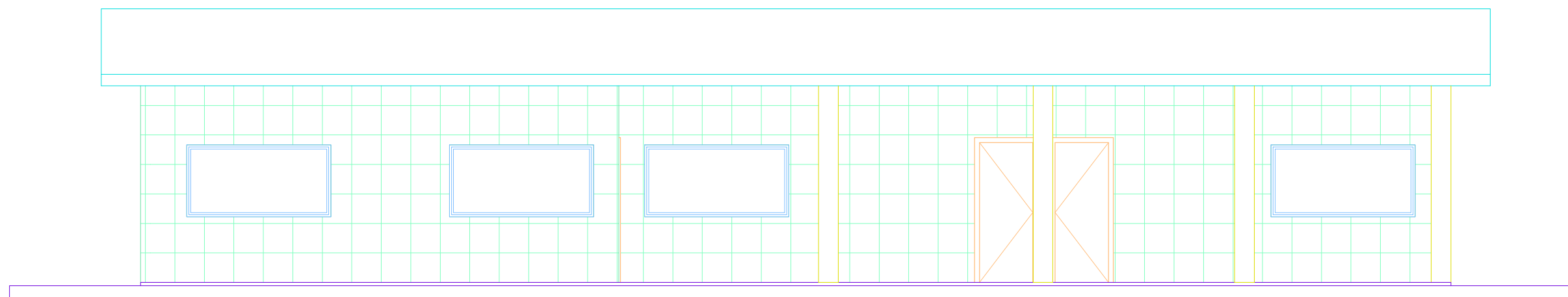
FACHADA PRINCIPAL escala 1/75
